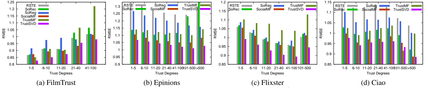
Figure 2: Performance comparison on users with different trust degrees ( d = 10 ) [best viewed in color]
